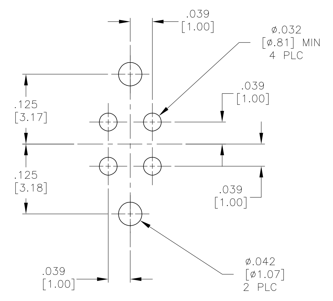
DETAIL T SCALE 10:1 2 PLC
