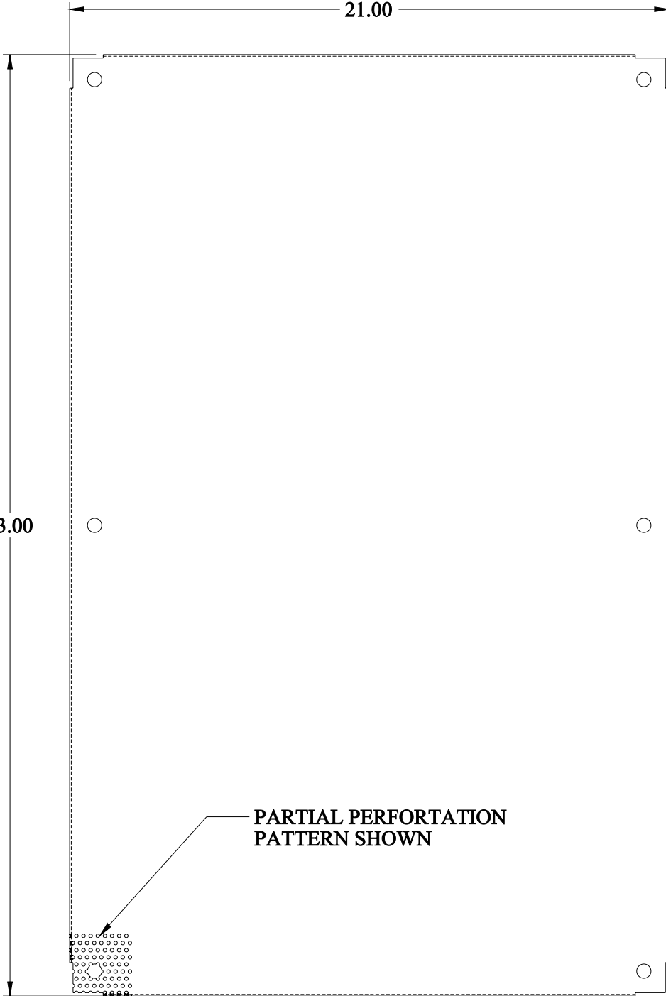
FRONT VIEW
