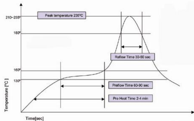
Figure 5 – Low Temperature Solder Reflow Thermal Profile
