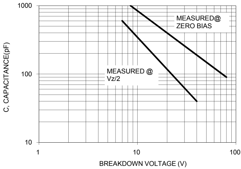
FIG.5 CAPACITANCE CURVE
