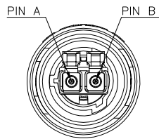
VIEW X-X (LC DUST COVERS NOT SHOWN)
