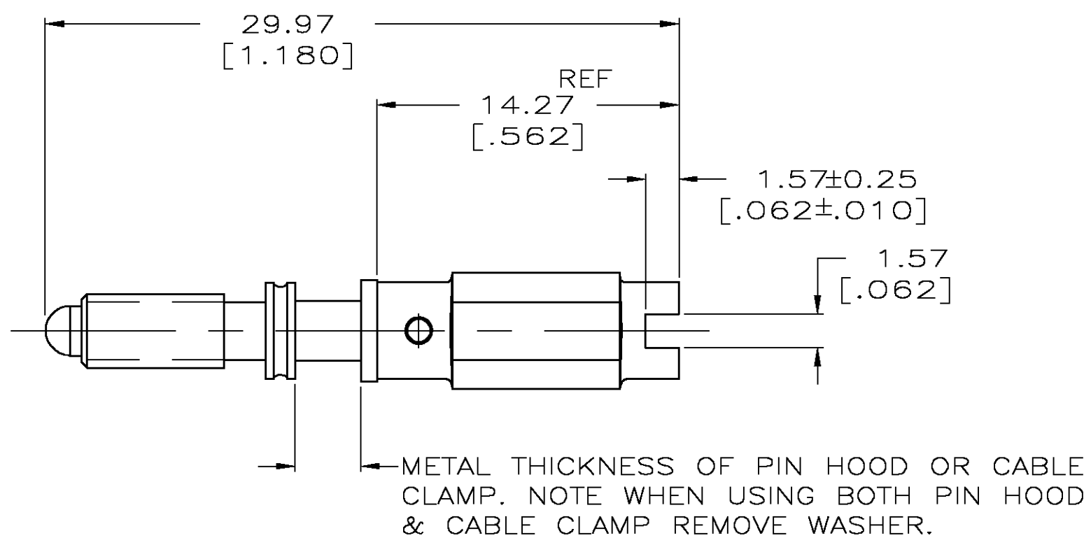
ASSEMBLED VIEW
