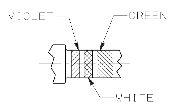
DETAIL X SCALE 10:1
