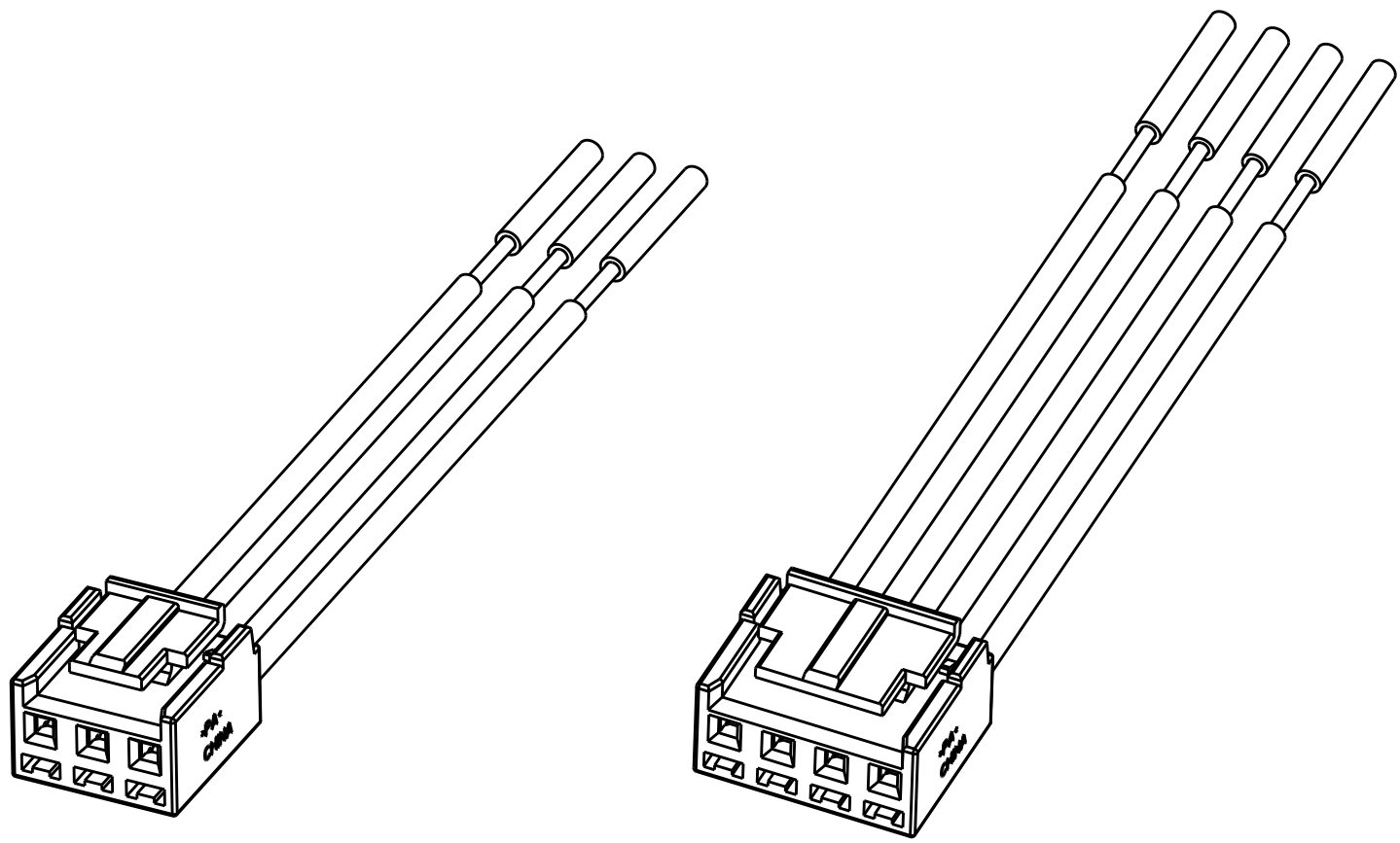
ISOMETRIC VIEW 4 POSITION
