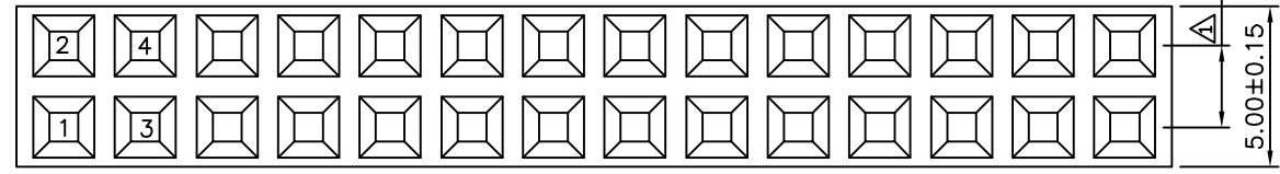
△ Recommended P.C.B. Layout(Top Side) (PCB Board Tolerance±0.05)
