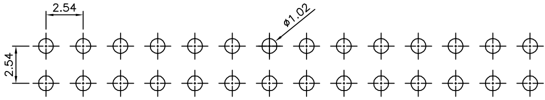
△ Recommended P.C.B. Layout(Top Side) (PCB Board Tolerance±0.05)
