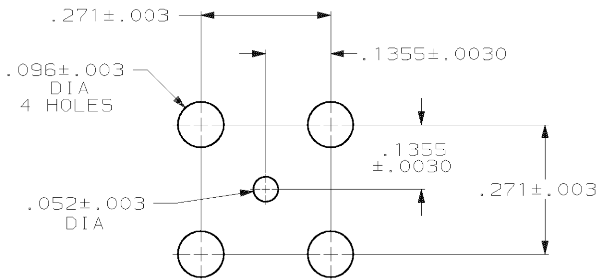
PCB CONFIGURATION
