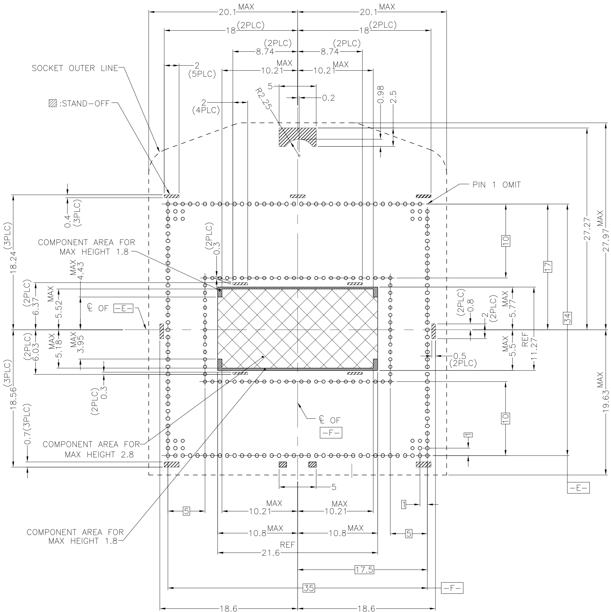
PCB LAYOUT 2229490-1 AS SHOWN
