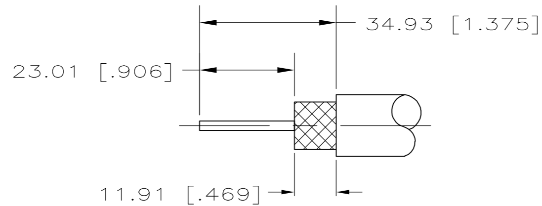
DETAIL B
