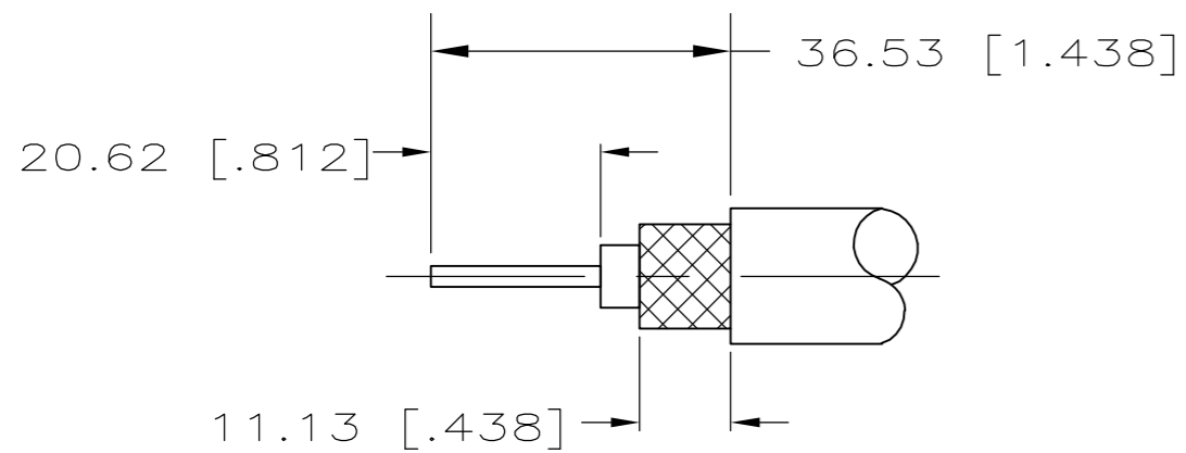
DETAIL A
