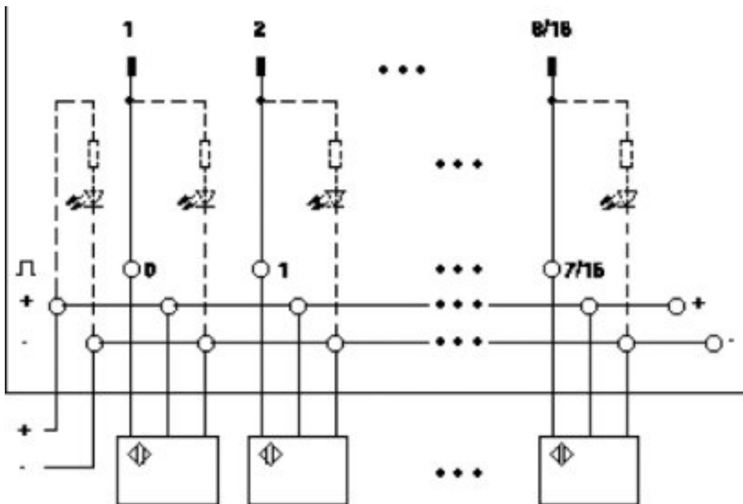
Circuit diagram
