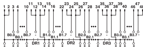
Circuit diagram
