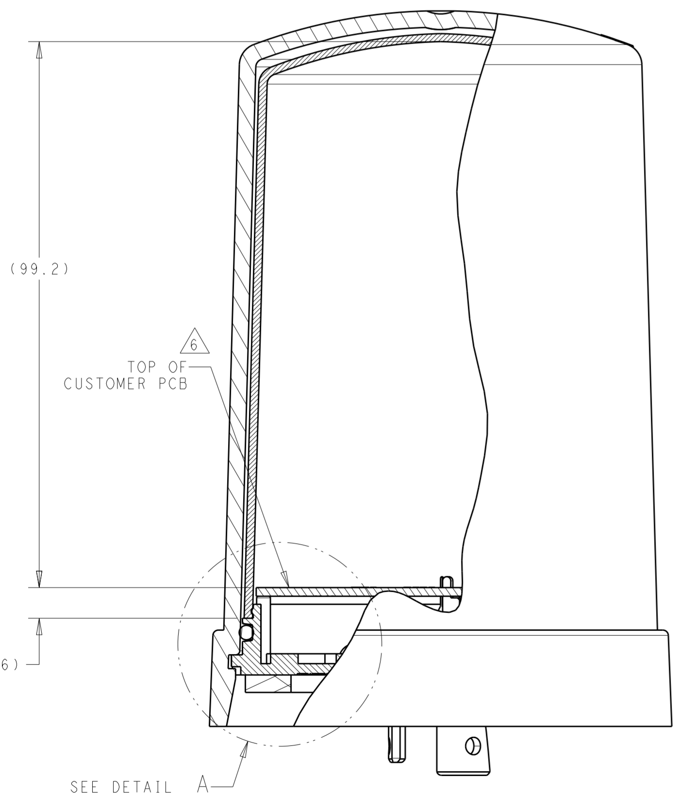
SECTION B-B SCALE 3:2
