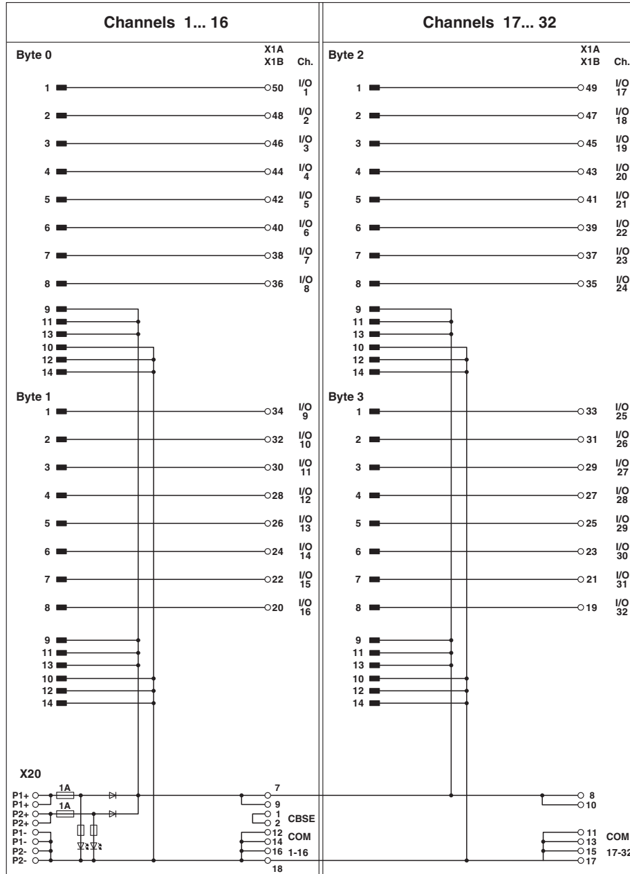
Circuit diagram
