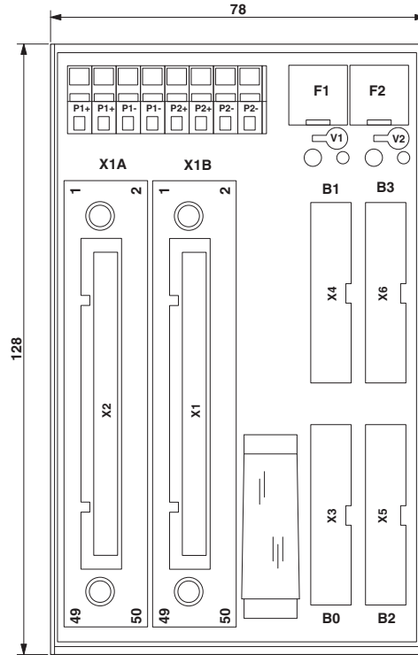
Dimensional drawing
