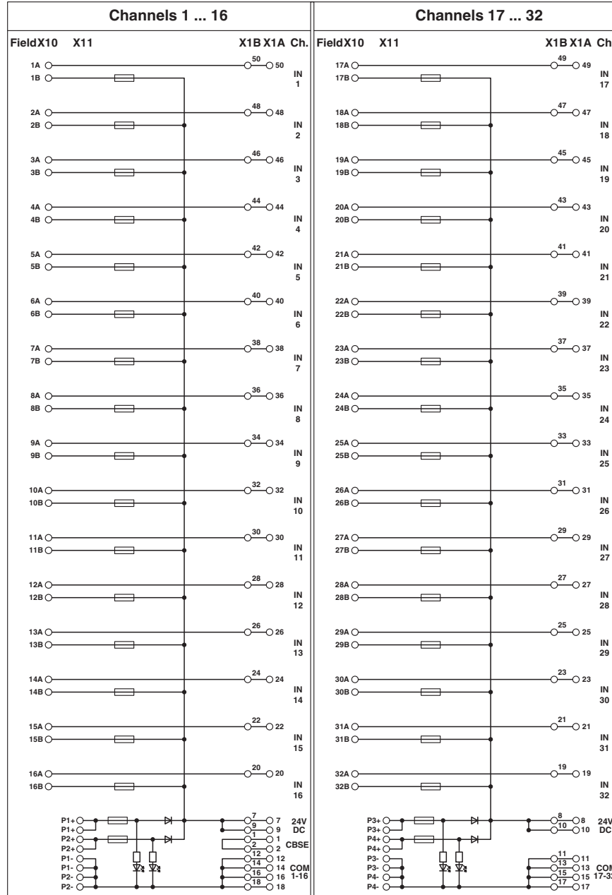
Circuit diagram
