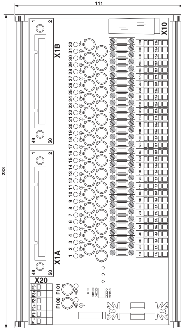
Dimensional drawing
