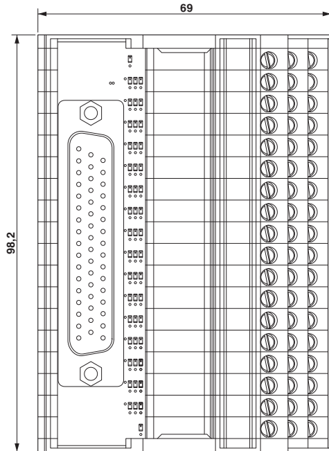
Dimensional drawing
