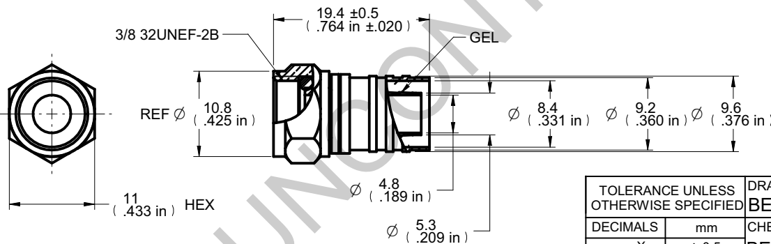
DIM OUTLINE
