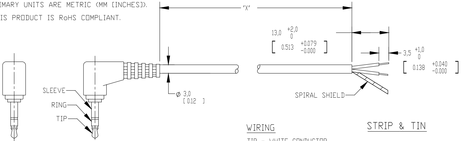
RA 2.5mm 3 CONDUCTOR PLUG
