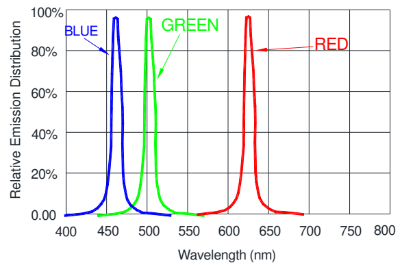
Wavelength Characteristics
