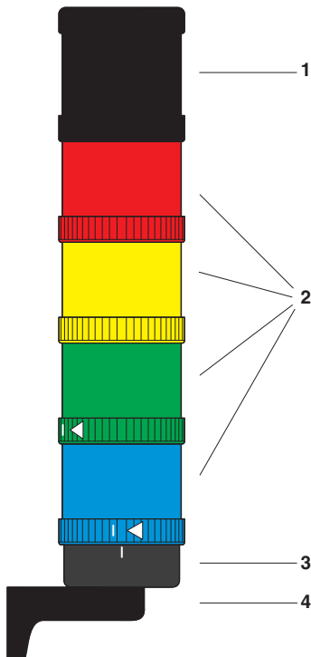
Figure 2 Example of a signal tower
