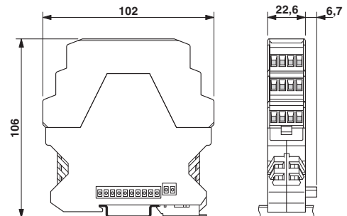
Dimensions of the electronic housing ME 22.5 flat.../BUS 5+2 and ME 22.5 flat.../BUS 10+2 with triple-level upper part
