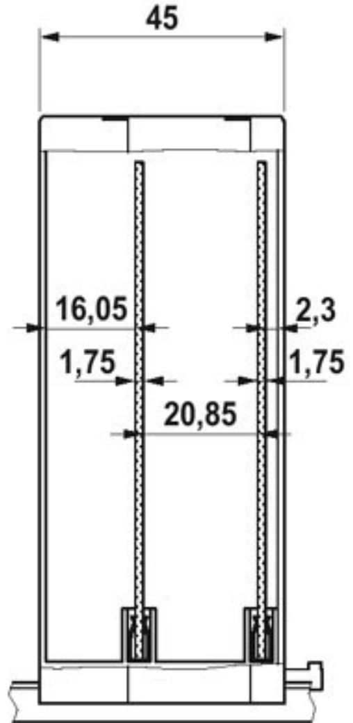
Dimensioned drawing
