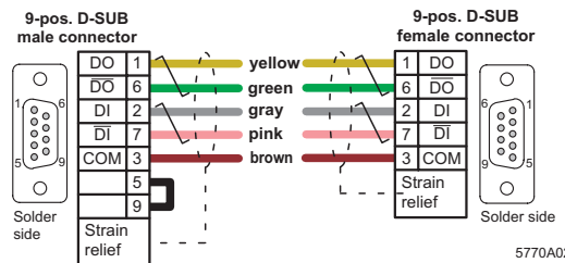
Figure 5 Example of a remote bus cable (cable type D9/D9)
