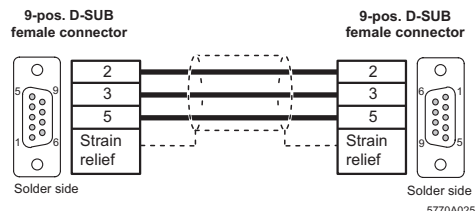
Figure 7 RS-232 cable for connection to a PC
