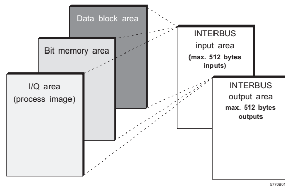
Figure 16 Source and destination areas for INTERBUS input/output data
