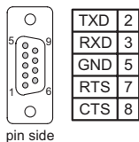
9-pos. D-SUB male connector
