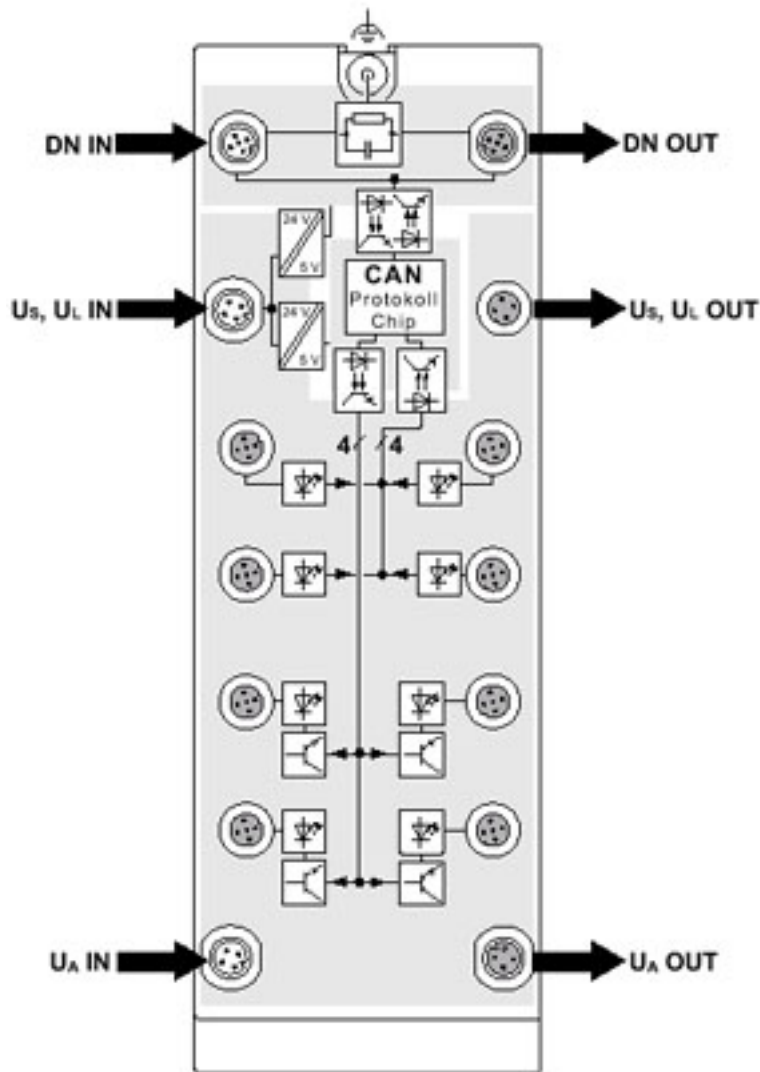
Block diagram
