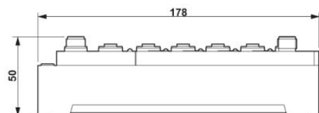
Dimensioned drawing
