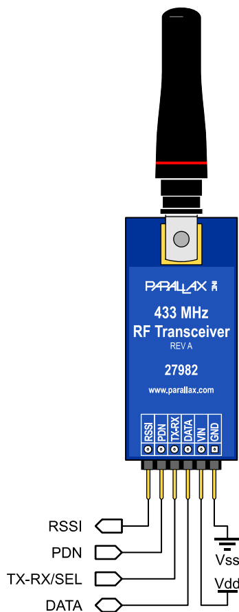
Figure 1: Pin Connections
