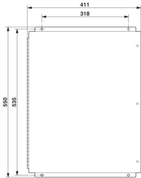
Dimensioned drawing
