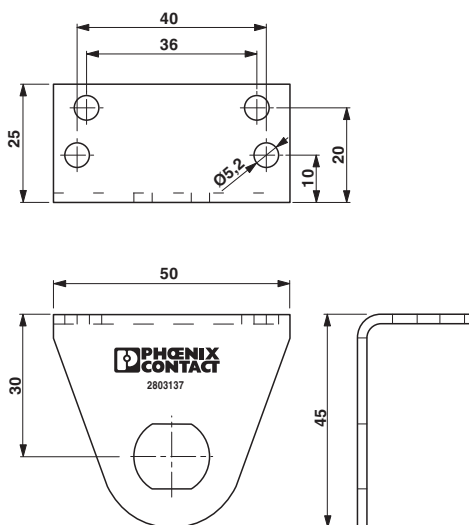
Dimensional drawing
