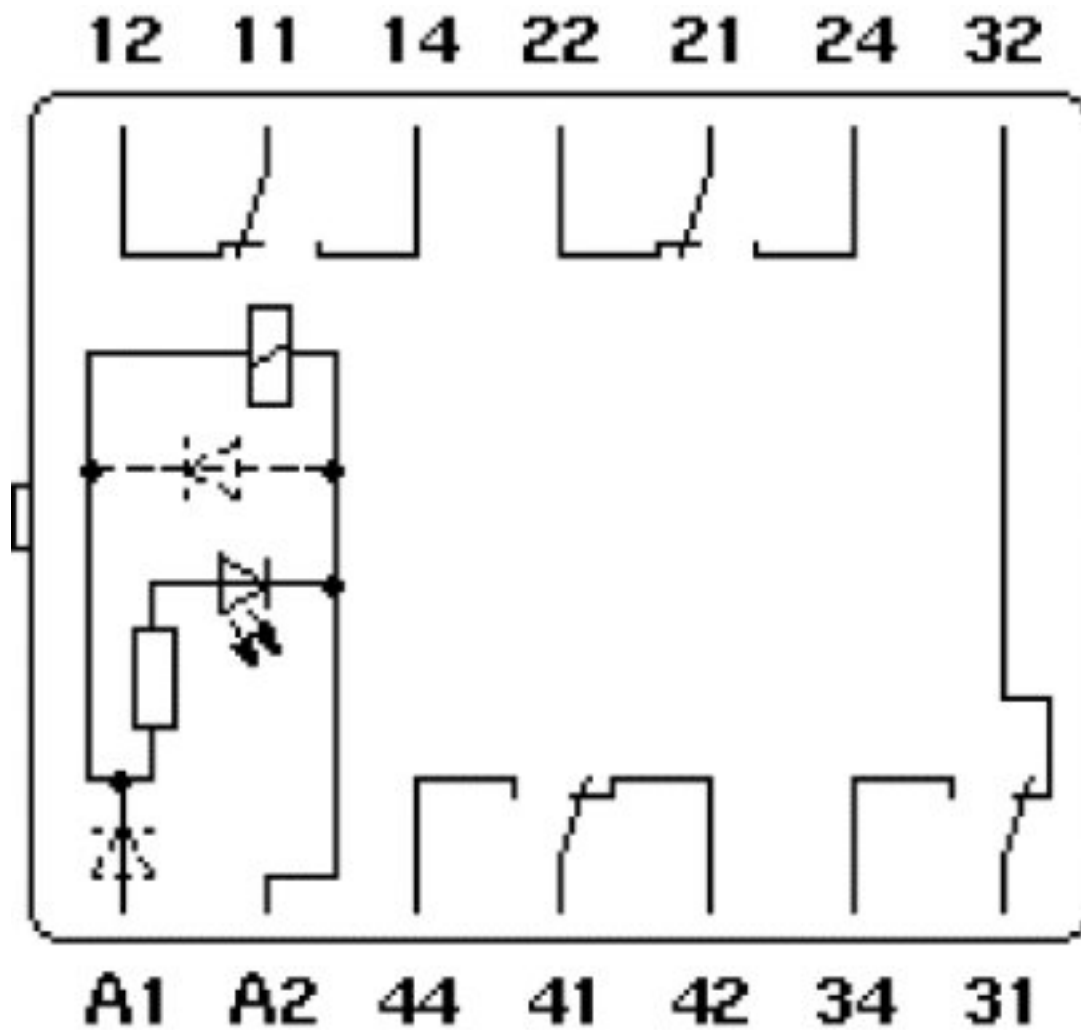
Circuit diagram
