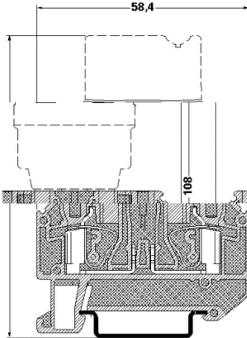
Dimensioned drawing
