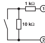
Figure 5 Switch contact with resistance circuit
