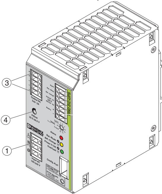
Figure 4 Connection
