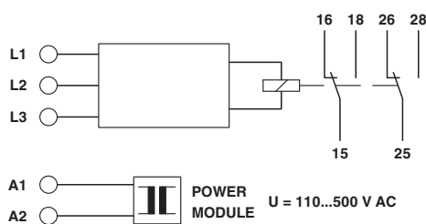
Block diagram
