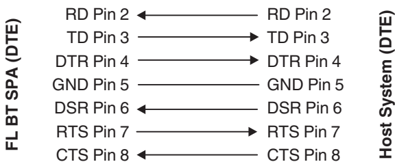
Figure 8 Assignment of 1:1 cables
