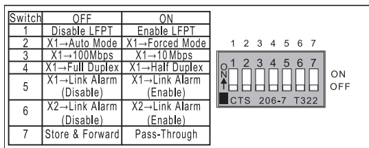
Figure 5 DIP switch
