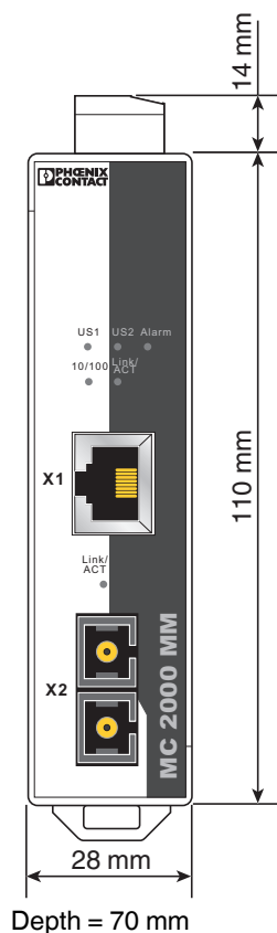
Figure 1 Housing dimensions
