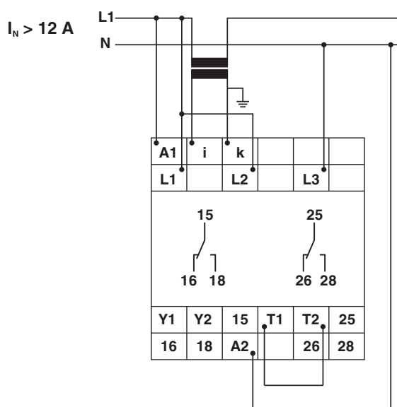
1~ 230 V connection with power module 230 V AC without error memory with current transformer
