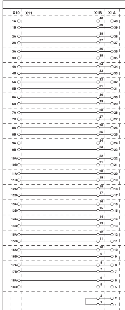
Circuit diagram
