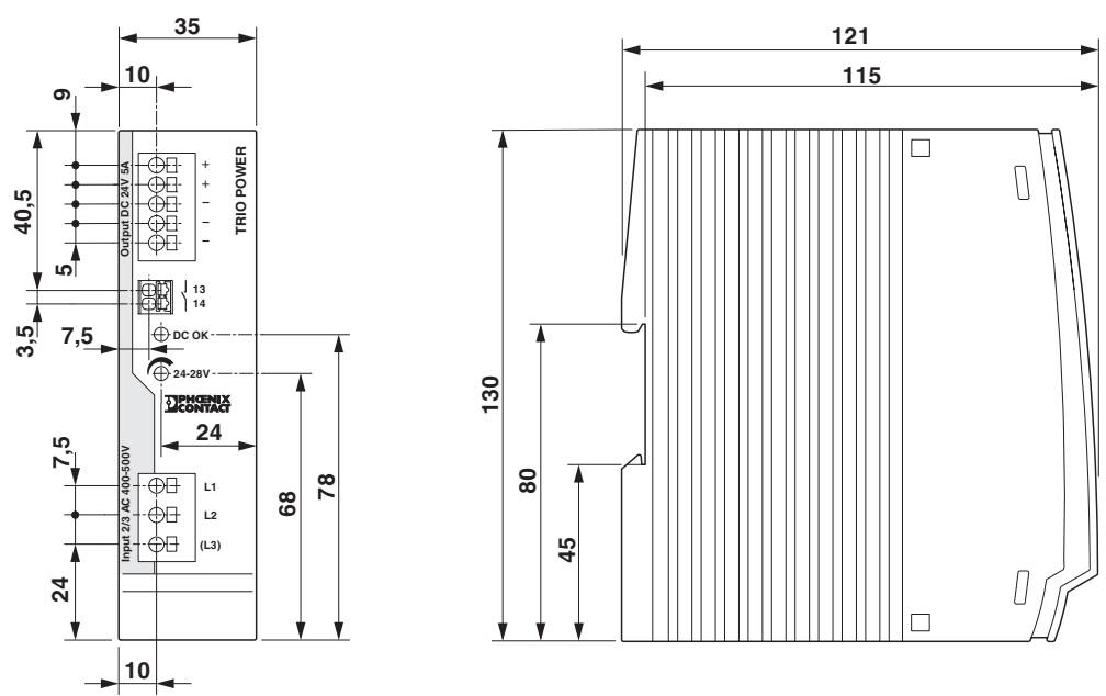
Figure 5 Device dimensions
