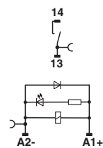
DC coils
