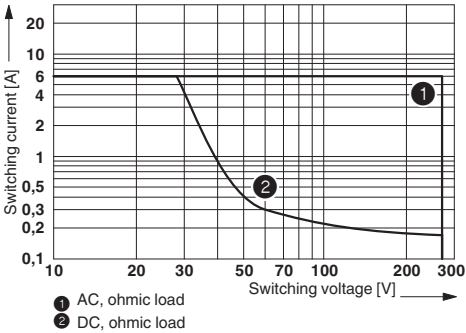
Interrupting rating
