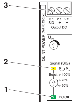
Figure 18 Position of signaling elements
