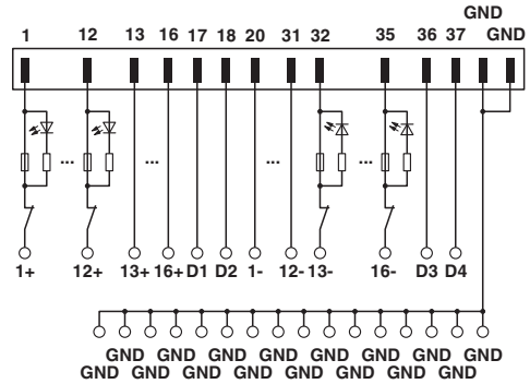
Circuit diagram
