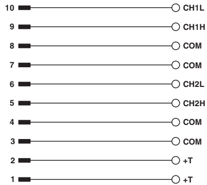
Circuit diagram
