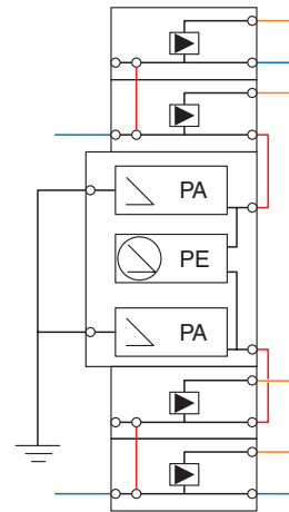
Circuit diagram
