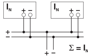
Figure 15 Redundancy operation
