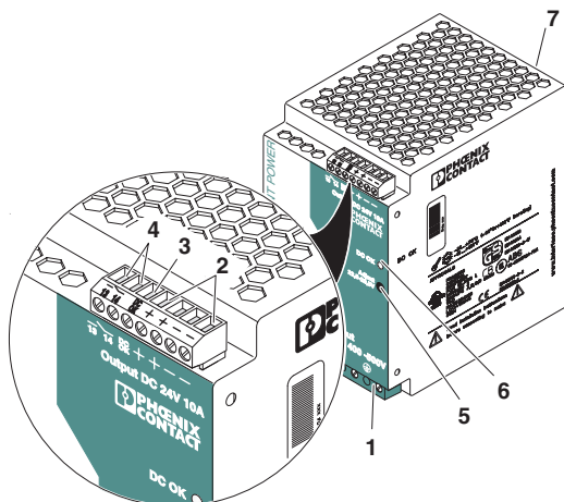
Figure 1 Operating elements
