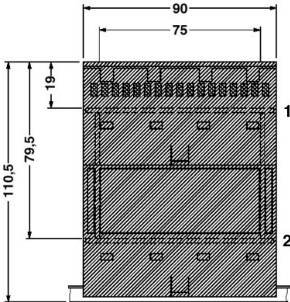
Dimensioned drawing
