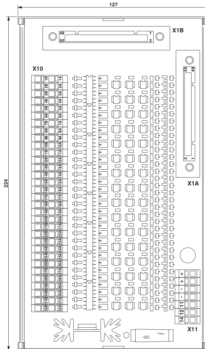
Dimensional drawing
